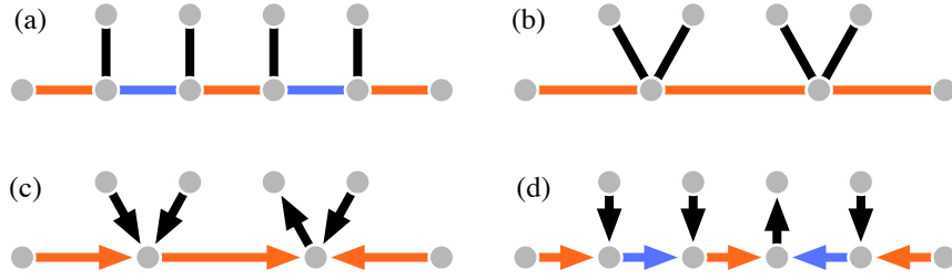
Figure 2: (a) Part of a high-girth 3-regular edge 3-coloured graph. (b) A 4-regular graph obtained by contracting all blue edges—note that the graph is not properly edge coloured. (c) With distributed LLL we can find a sinkless orientation in the 4-regular graph. (d) We can now orient each blue edge greedily to obtain a sinkless orientation of the original graph.
