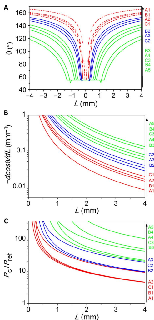
Fig. 4. Mechanistic understanding. (A to C) Calculated oil contact angle \theta (A), wettability gradient -d(\cos \theta)/dL (B), and breakthrough pressure P_c/P_{ref} (C) curves as functions of L on the 12 patterned surfaces. Different curve colors correspond to the three modes of droplet motion. The red curves in (A) are shown in dashed lines because oil droplets tend to collapse into the Wenzel state in this regime.
