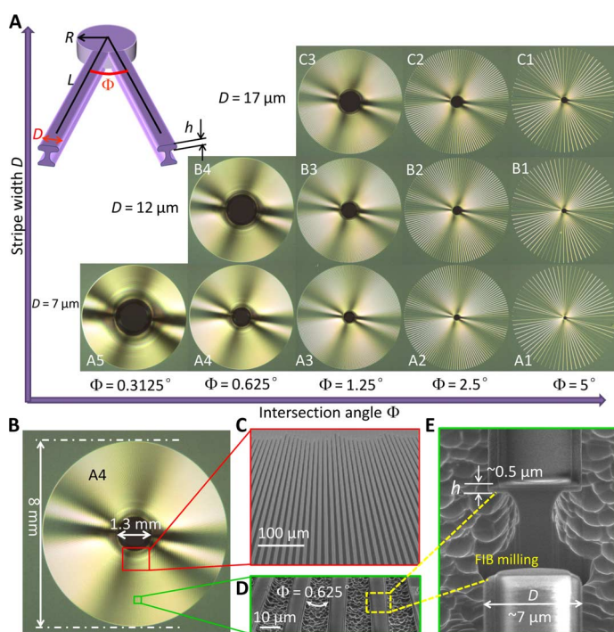
Fig. 2. The fabricated patterns composed of radially arrayed undercut microstrips. (A) Photographs of 12 samples with systematically varied parameters. Inset: Schematic illustration of the two neighboring stripes with the undercut structure. D is the stripe width, \Phi is the intersection angle between two neighboring stripes, R is the radius of the central circle formed by intersection of the stripes, h is the undercut thickness, and L is the distance to the center. (B to E) Structure details of a typical A4 sample. (C) Scanning electron microscope (SEM) image near the center shows radially arrayed microstrips. (D) Magnified image of the radial stripes far from the center. (E) Cross-sectional view of an individual stripe reveals the undercut profile. The stripe was locally removed by focused ion beam (FIB) milling to expose the cross-sectional morphology.
