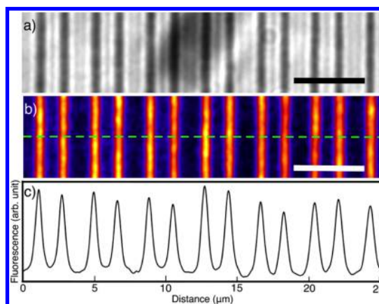
Figure 1. (a) Bright-field microscopy image of a fabricated line array in 50% Ag@PMAA samples ( I_{dlw} = 80 GW/m 2 , \lambda_{dlw} = 780 nm). Scale bar = 5 \mu m. (b) Corresponding fluorescence images of the same area ( \lambda_{exc} = 473 nm). (c) Fluorescence intensity profile across the marked line in (b).
