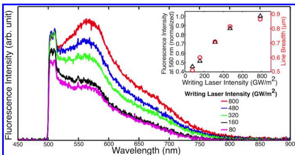
Figure 4. Fluorescence emission spectra ( \lambda_{\text{exc}} = 473 \text{ nm} ) recorded from the structures written at I_{\text{dlw}} : 80, 160, 320, 480, and 800 \text{GW/m}^2 . Inset shows the fluorescence intensity at 560 nm and the corresponding breadth of the fluorescent grooves against writing power.
