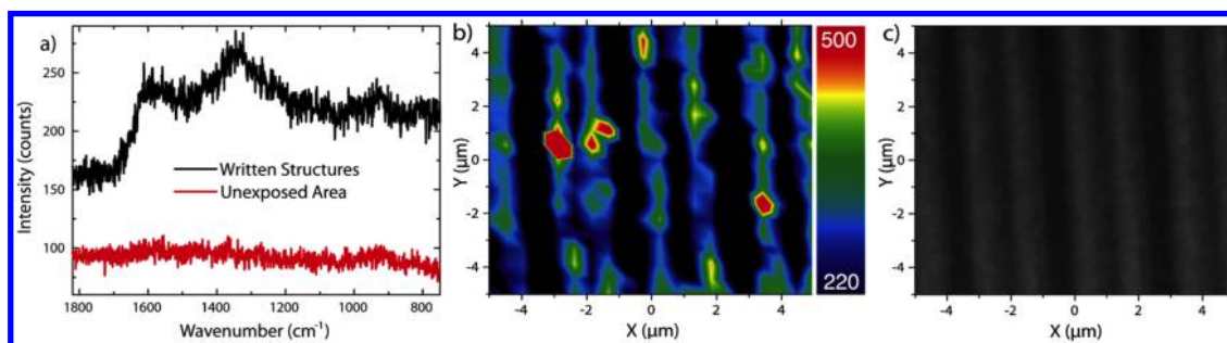
Figure 6. (a) Raman spectra detected from the written structures (black curve) and unexposed regions (red curve). (b) Raman microscopy image of the written structures at 1340\text{ cm}^{-1} . Color scale bar corresponds to the Raman signal counts. (c) Bright-field microscopy image of the corresponding area.
