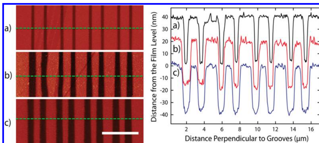
Figure 3. AFM images of structures written with I_{\text{dlw}} of (a) 80 GW/m 2 , (b) 240 GW/m 2 , and (c) 480 GW/m 2 in 50% Ag@PMAA samples. Scale bar = 5 \mu\text{m} . The full width at half-maxima of the grooves measured from line-cut topography profiles (right) are (a) 380 \pm 40 nm, (b) 710 \pm 120 nm, and (c) 850 \pm 80 nm, respectively. For clarity, the line profiles for (a) and (b) have been vertically shifted by 40 and 20 nm, respectively.
