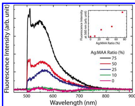
Figure 2. Fluorescence emission spectra of laser-written silver nanoclusters in Ag@PMAA films with Ag/MAA ratios ranging from 0 to 75% ( \lambda_{exc} = 473 nm). Inset shows the Ag concentration dependence of the fluorescence intensity at 560 nm in Ag@PMAA samples.
