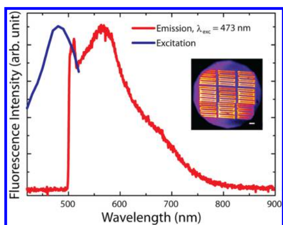
Figure 5. Excitation (blue curve) and emission (red curve) spectra ( \lambda_{\text{exc}} = 473 \text{ nm} ) obtained from fluorescent silver nanoclusters in microstructures (inset). The excitation spectrum was measured by evaluating the total emission counts between 532 and 650 nm. Inset shows the fluorescence image of the investigated microstructures. Scale bar = 5 \mu\text{m} .
