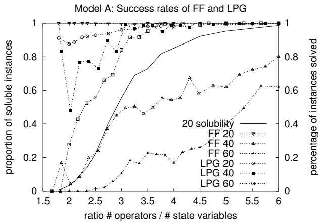
Figure 4: Percentage of soluble problem instances with 20, 40 and 60 state variables FF and LPG solved in 10 minutes. For 40 and 60 state variables the curves depict the proportion of the number of instances solved by FF and LPG to the number of instances solved by SP. The success rates on 40 and 60 state variables is an upper bound because SP very likely missed some of the soluble instances.
