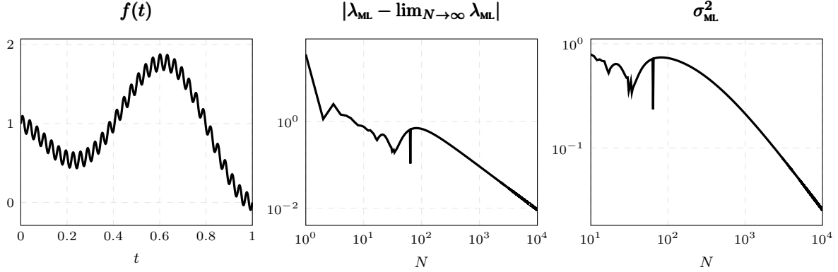
Fig. 1: The differentiable function (10) on [0, 1] and the behaviour of the maximum likelihood estimates \lambda_{\text{ML}} and \sigma_{\text{ML}}^2 in (5) and (6) as functions of N .
