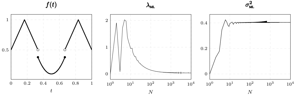
Fig. 2: The discontinuous function (11) on [0, 1] and the behaviour of the maximum likelihood estimates \lambda_{\text{ML}} and \sigma_{\text{ML}}^2 in (5) and (6) as functions of N .
