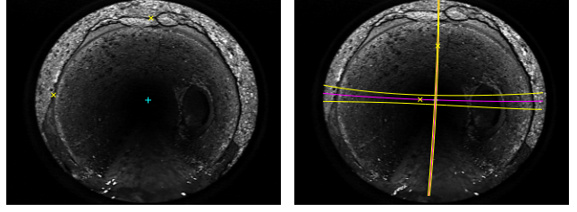
Figure 1: Estimated epipolar geometry for two fish-eye images. Two points in the first image are chosen (yellow crosses) and their epipolar curves (magenta curves) are plotted to the second image. The yellow curves are the epipolar envelopes. The envelope of the horizontal curve is broad because a very large value of k^2 = 1000 was chosen in (9) in order to better illustrate the error bounds. The narrow confidence interval of the vertical curve is the 95 % envelope that corresponds to a value k^2 = 5.99 .
