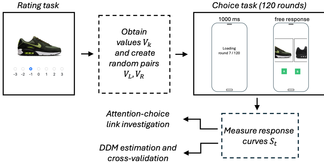
Figure 2: Experimental Design for the Consumer Choice Study
