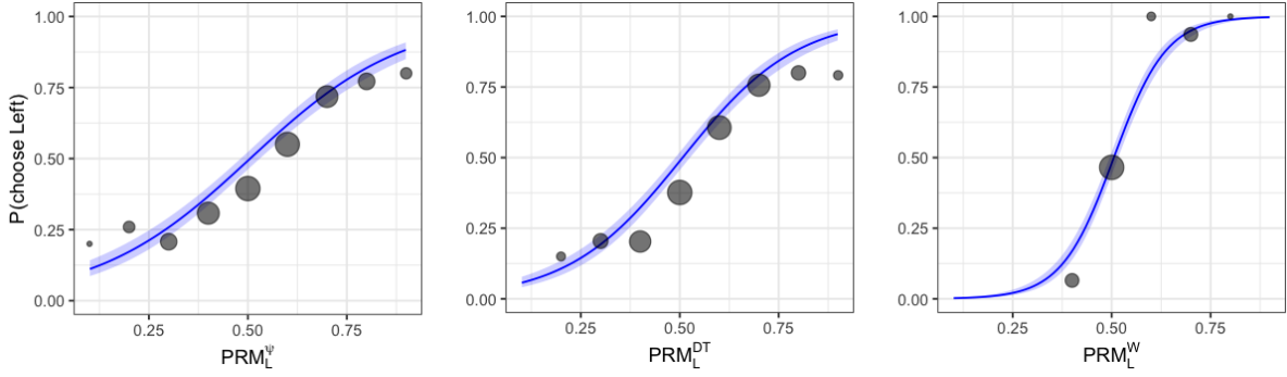
Notes. The blue curve represents logit-GLMM estimations when the data are restricted by condition V_L = V_R , see Table 1 for results with the full data set. Shaded ribbons are 95% confidence intervals. In each panel, points depict group means of choice probabilities in 9 different bins of PRM values at increments of 0.1, and each point is plotted at the bin’s upper boundary. The right panel contains fewer points because the data are concentrated on fewer bins. Point size represents the relative size of each bin. In the middle panel, one point is omitted because its bin contained only a single value.
