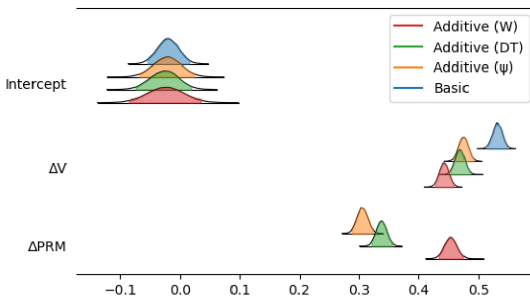
Figure 6: Marginal Posterior Distributions for the Basic and Additive Model Coefficients (Equation (8))
