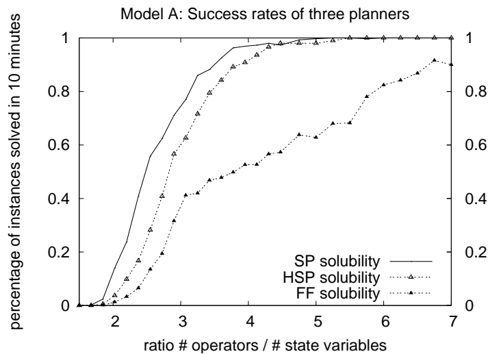
Fig. 14. Percentage of problem instances with 40 state variables solved in 10 minutes by our planner, HSP and FF.
