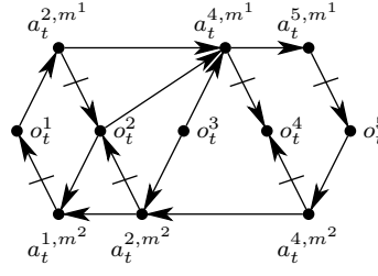
Fig. 2. A linear-size encoding of interference constraints
