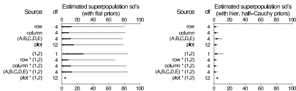
Figure 15.5 Posterior medians, 50%, and 95% intervals for standard deviation parameters \sigma_k estimated from a split-plot latin square experiment. (a) The left plot shows inferences given uniform prior distributions on the \sigma_k 's. (b) The right plot shows inferences given a hierarchical half-Cauchy model with scale fit to the data. The half-Cauchy model gives much sharper inferences, using the partial pooling that comes with fitting a hierarchical model.
