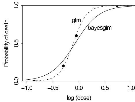
Figure 16.3 Estimates from maximum likelihood and Bayesian logistic regression with the recommended default prior distribution for the bioassay example (data in Table 3.1 on page 74). In addition to graphing the fitted curves (at right), we show raw computer output to illustrate how our approach would be used in routine practice. The big change in the estimated coefficient for z.x when going from glm to bayesglm may seem surprising at first, but upon reflection we prefer the second estimate with its lower coefficient for x , which is based on downweighting the most extreme possibilities that are allowed by the likelihood.
