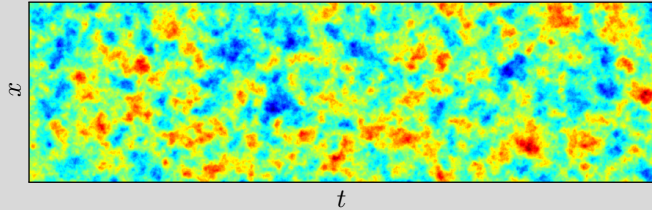
Fig. 3: A random realization simulated by the state space model in Equation (36).
