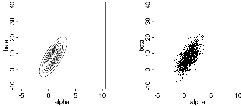
Figure 4.1 (a) Contour plot of the normal approximation to the posterior distribution of the parameters in the bioassay example. Contour lines are at 0.05, 0.15, . . . , 0.95 times the density at the mode. Compare to Figure 3.3a. (b) Scatterplot of 1000 draws from the normal approximation to the posterior distribution. Compare to Figure 3.3b.
