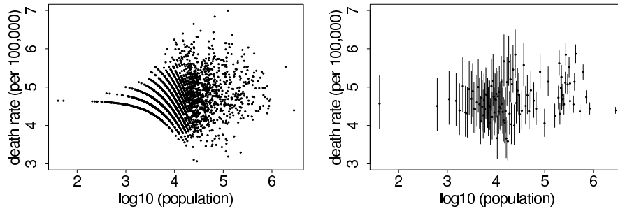
Figure 2.9 (a) Bayes-estimated posterior mean kidney cancer death rates, E(\theta_j|y_j) = \frac{20+y_j}{430,000+10n_j} vs. logarithm of population size n_j , the 3071 counties in the U.S. (b) Posterior medians and 50% intervals for \theta_j for a sample of 100 counties j . The scales on the y-axes differ from the plots in Figure 2.8b.
