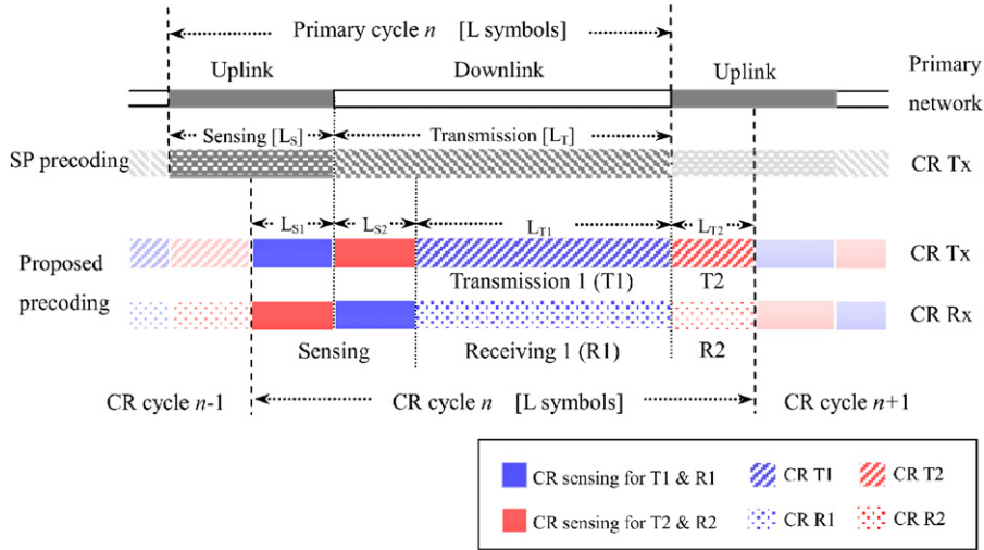
Fig. 2. System diagram for the proposed precoding schemes.
