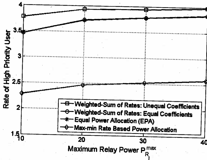
Figure 4. Rate of high priority users versus P_r^{\max}
