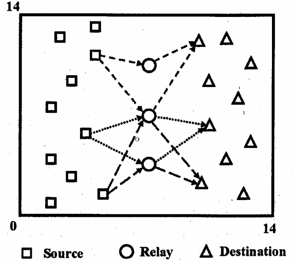
Figure 3. Multi-user wireless relay network
