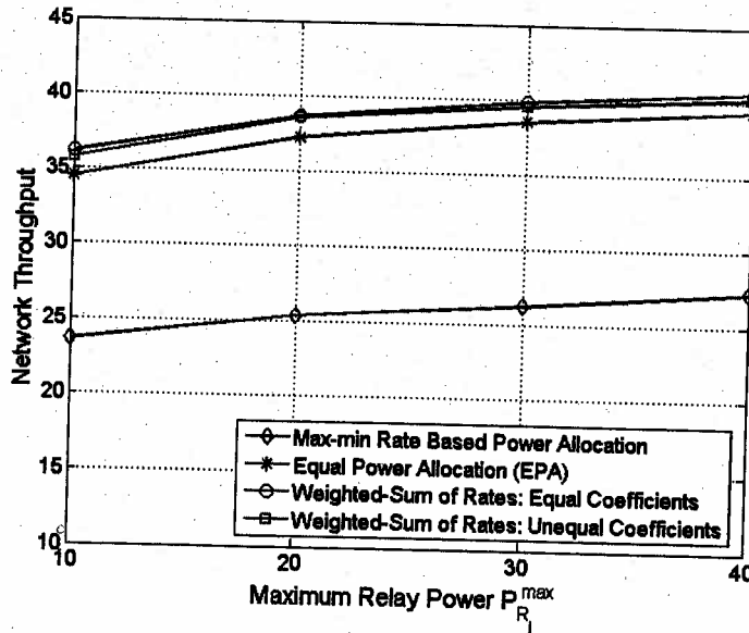
Figure 5. Network throughput versus P_r^{\max}
