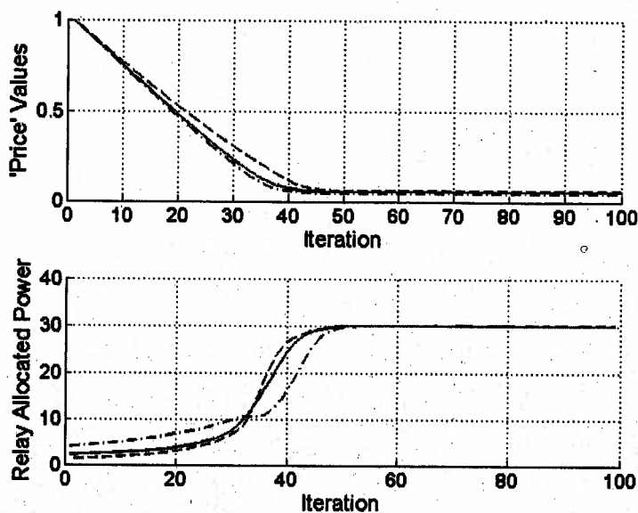
Figure 6. Evolution of 'price' values and powers allocated at each relay
