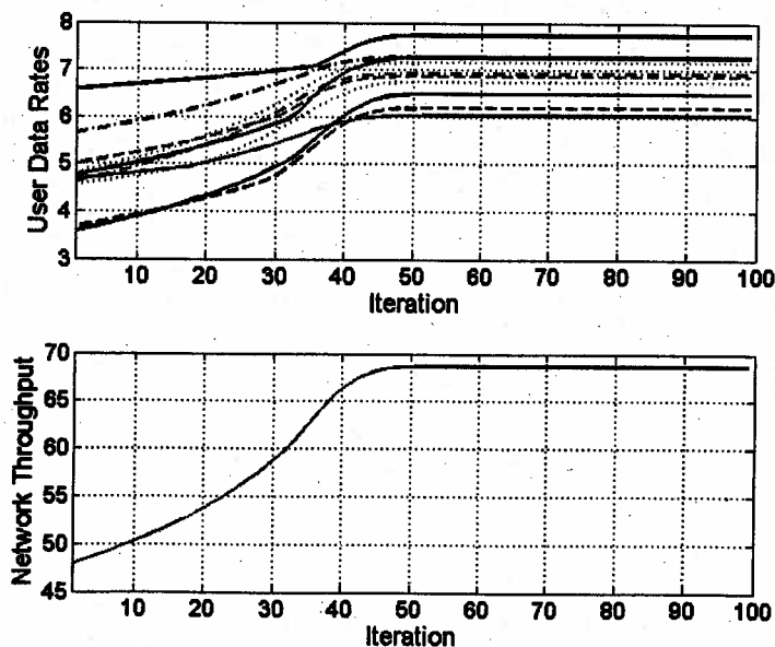
Figure 7. Evolution of data rate for each user and user sum rate
