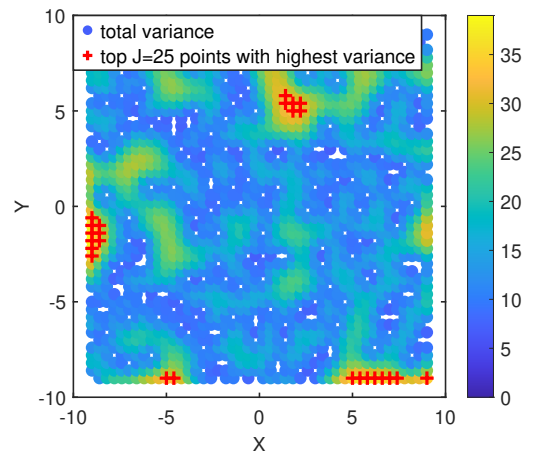
Fig. 2. The heatmap of estimation variance. Landmarks are white colored, and high variance points are red colored.
