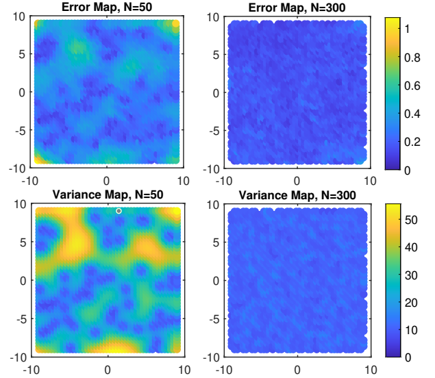
Fig. 6. Heatmap for Kriging interpolation estimation error and variance with 50 random points and 300 points found by adaptive sampling.
