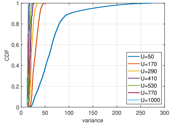
Fig. 5. The distribution of total variance estimation for adaptive sampling.
